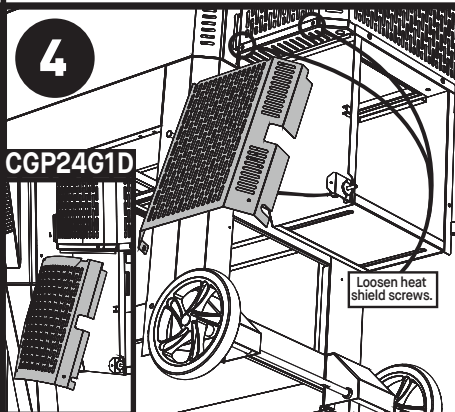
Remove the front heat shield.
