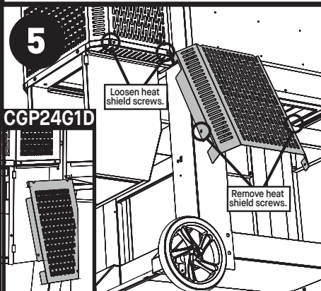
Remove the ash rear heat shield.
