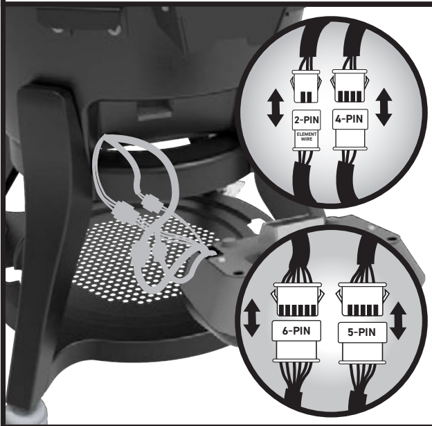
Disconnect the wire harness from the rear module. Use caution do not apply tension on the wire harness.
